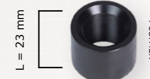
Schutzkappe Ø 27/29 mm Protection cap Ø 27/29 mm (M19x1)
