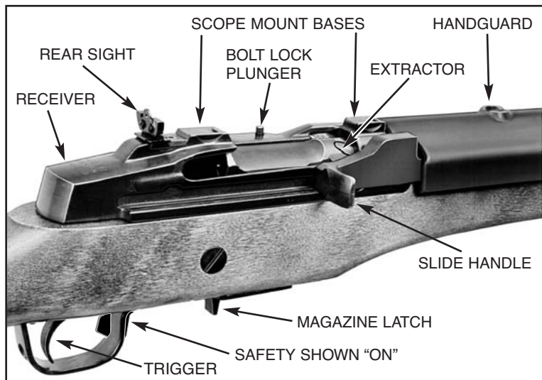
Figure 2. In this illustration the frequently used operating components are identified. Note that the safety is rearward in the trigger guard and is therefore in its "ON" (safe) position.
