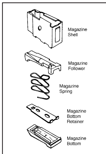
Figure 16. Exploded view of the Mini Thirty magazine components. This illustration is included to show the relationship and names of the magazine components.
